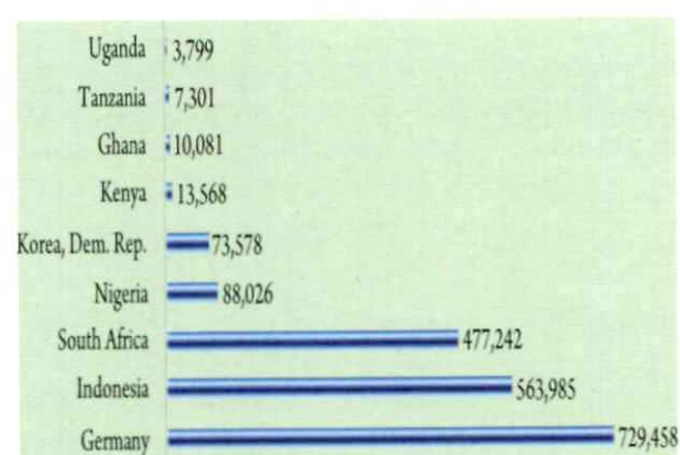
Figure 13.2: Carbon dioxide emissions, 2011 (in thousand metric tonnes)
