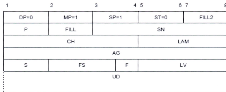
Figure 5-3. CALL REQUEST by ADLP packet
