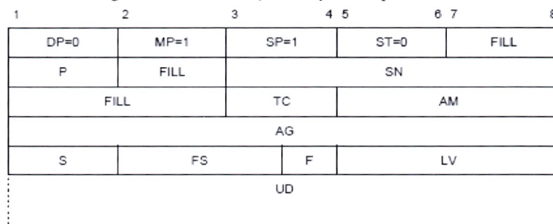
Figure 5-3. CALL REQUEST by ADLP packet
