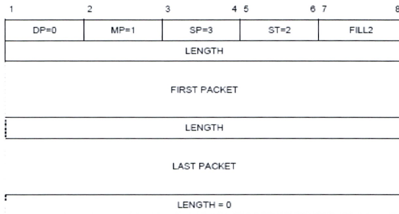
Figure 5-20. MULTIPLEX packet
