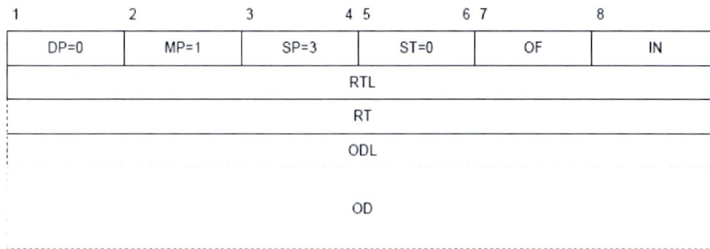
Figure 5-19. ROUTE packet
