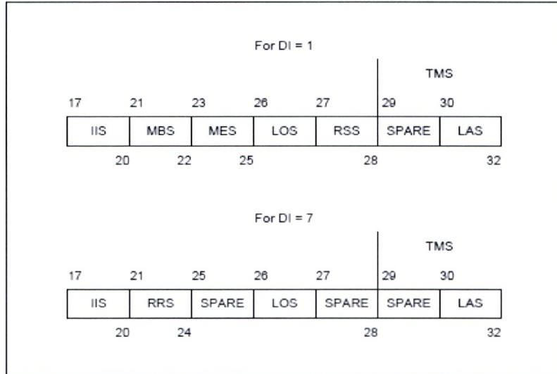
Figure 5-1. The SD field structure
