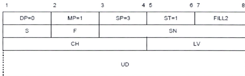
Figure 5-12. INTERRUPT packet
