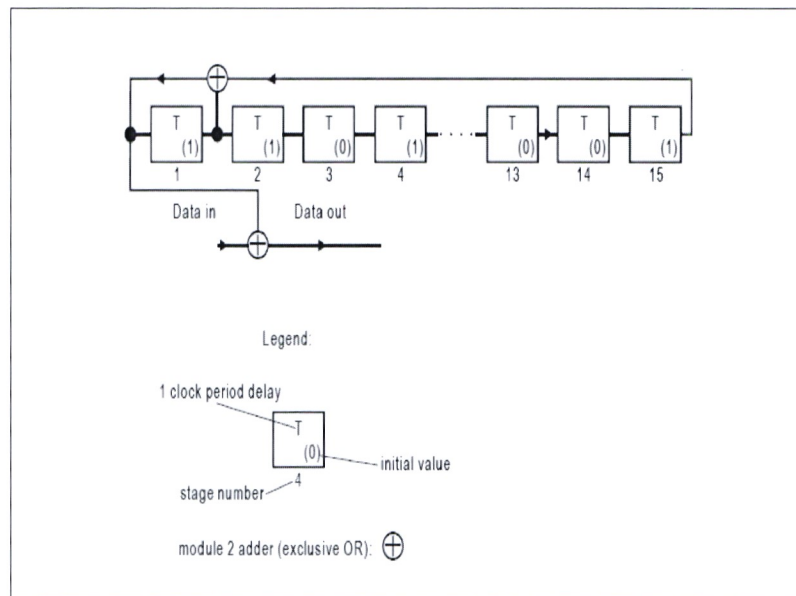
Figure 6-2 PN generator for bit scrambling
