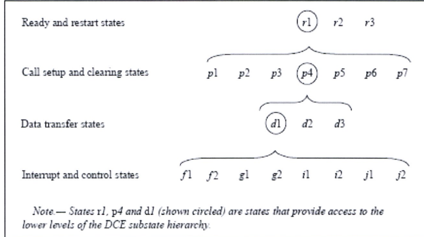
Figure 5-2. DCE substate hierarchy
