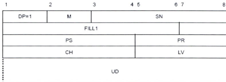
Figure 5-11. DATA packet
