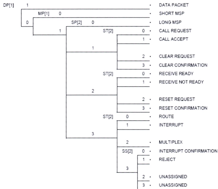
Figure 5-23. Control fields used in MODE S packets
