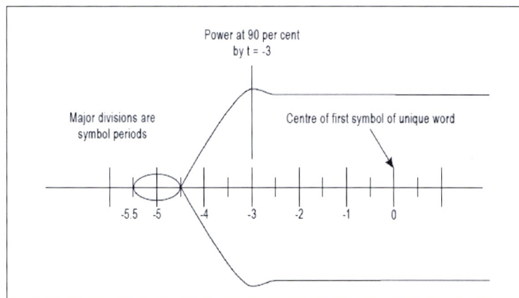
Figure 6-1 Transmitter power stabilization
