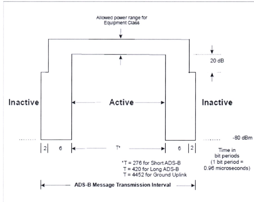
Figure 12-2. Time/amplitude profile of UAT message transmission
