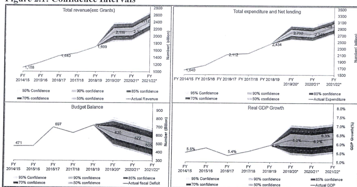
Figure 2.1: Confidence Intervals
