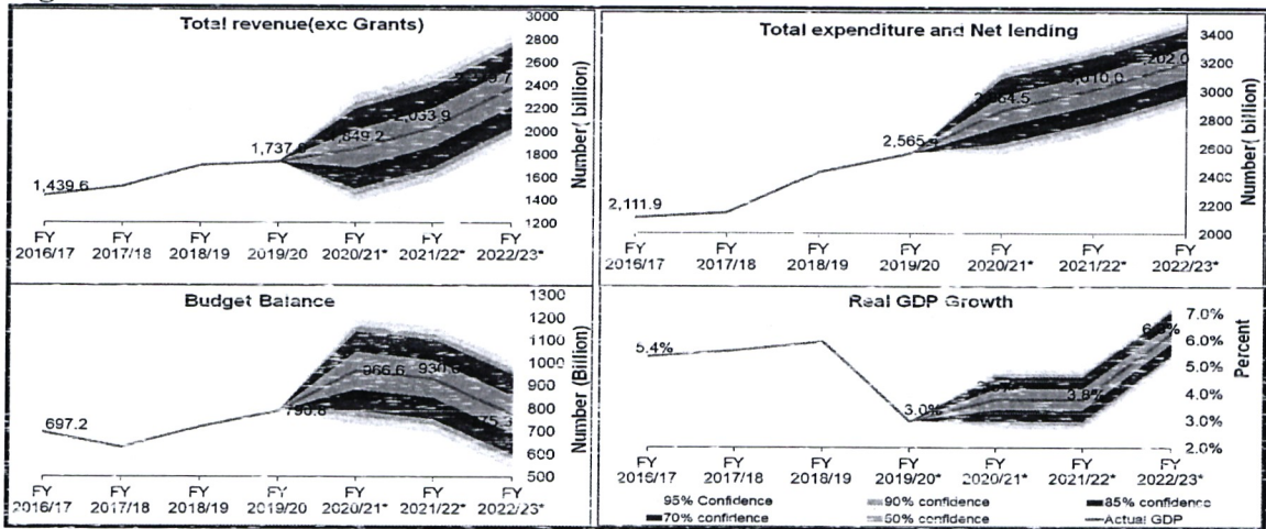
Figure 20: Confidence Intervals
