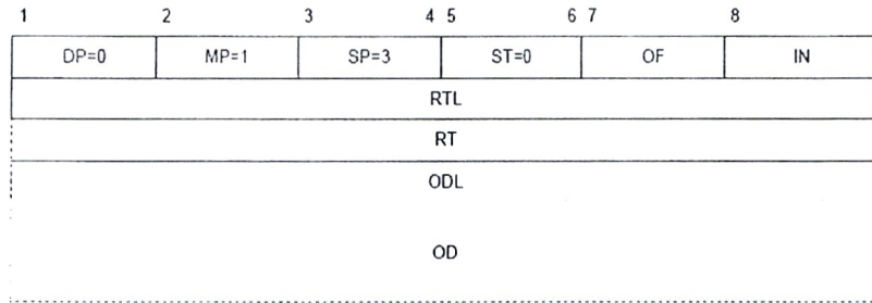
Figure 5-19. ROUTE packet
