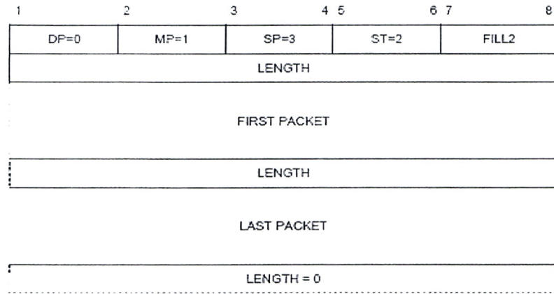
Figure 5-20. MULTIPLEX packet
