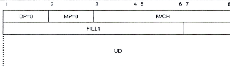
Figure 5-20. MULTIPLEX packet
