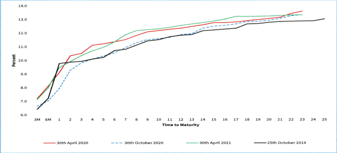
Chart 6c: Government Securities Yield Curve
