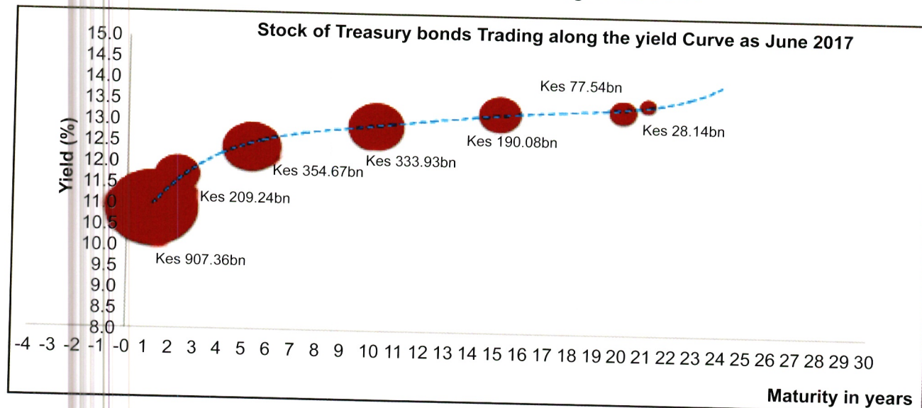
Figure 2-6: Stock of Treasury Bonds Along the June 2017 Average Yield Curve
