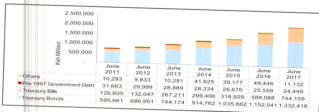
Figure 2-1: Stock of Domestic debt
