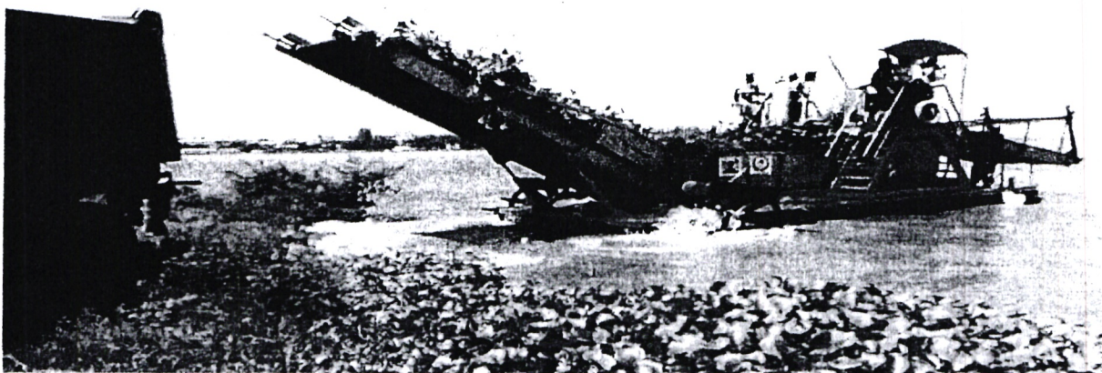
Picture 9: Test run of the water hyacinth harvester procured by LVEMP II Kenya for mechanical removal of the weed
