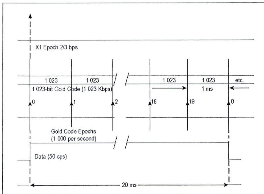
Figure B-1. C/A code timing relationships
