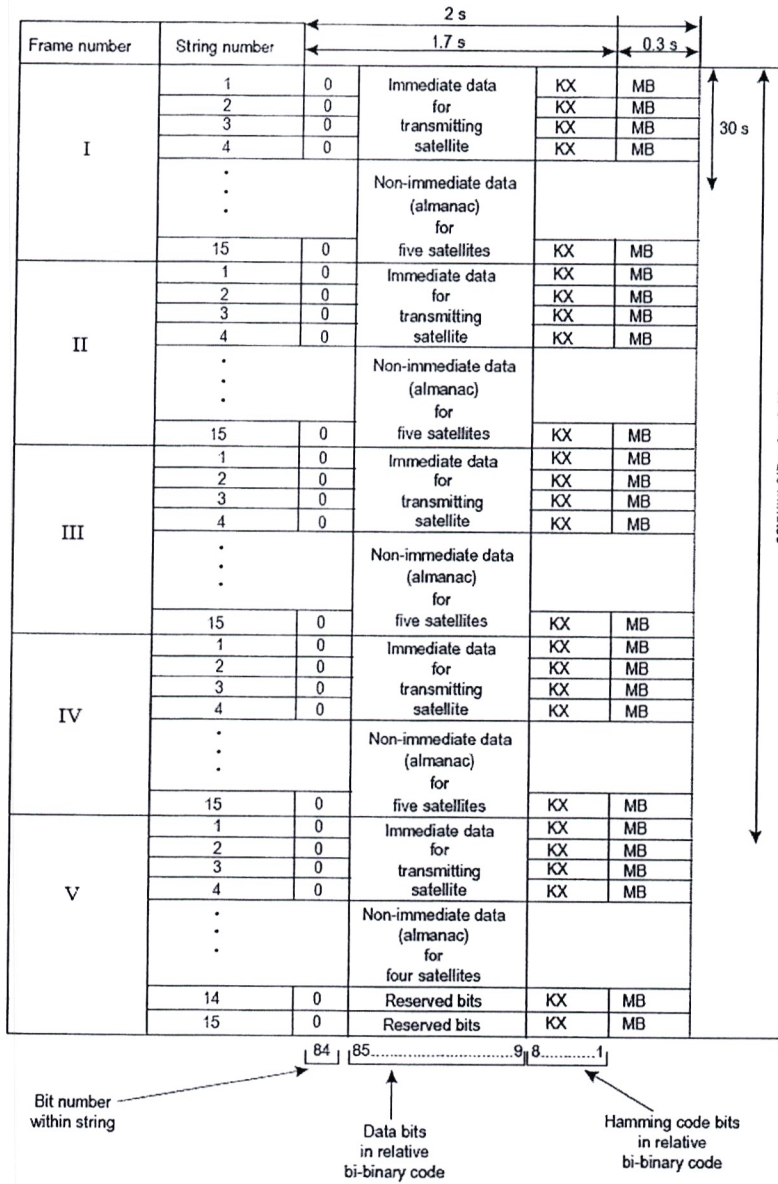
Figure B-7. Superframe structure
