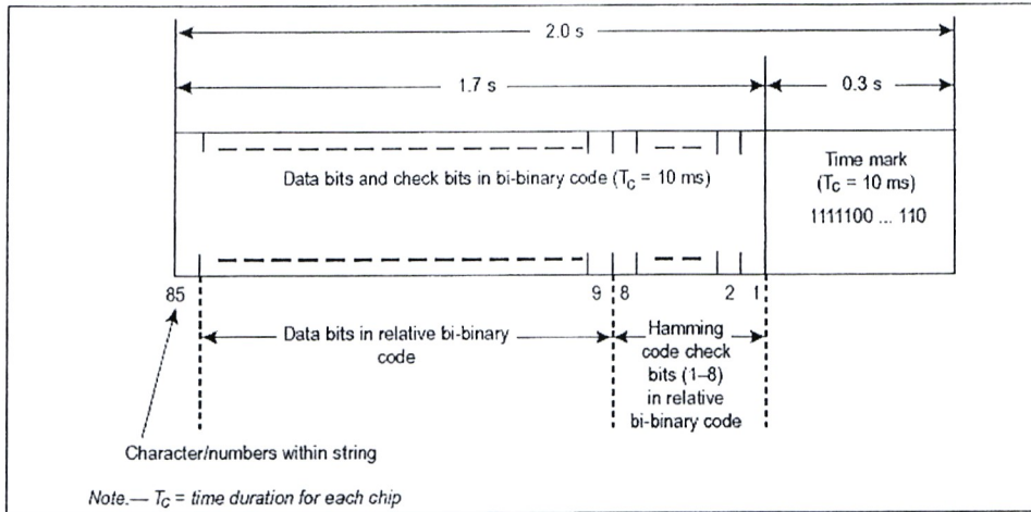
Figure B-10. Data string structure
