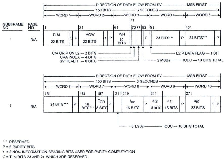
Figure B-6. Data format (1 of 11)
