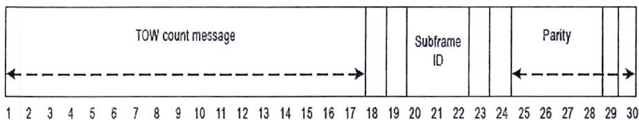
Figure B-4. HOW format
