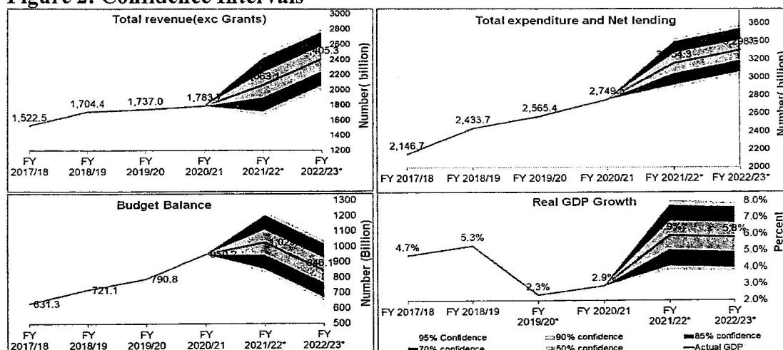
Figure 2: Confidence Intervals
