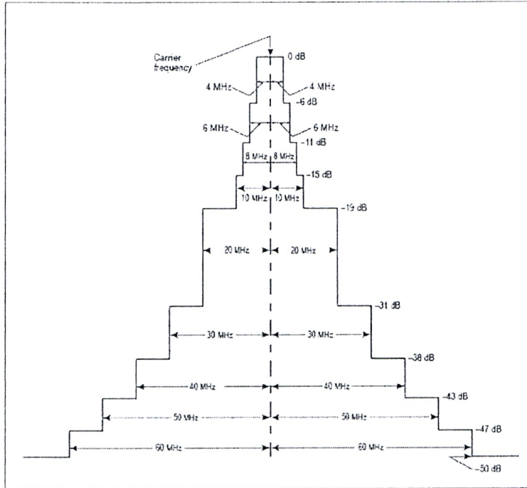
Figure 3-2. Required spectrum limits for interrogator transmitter
