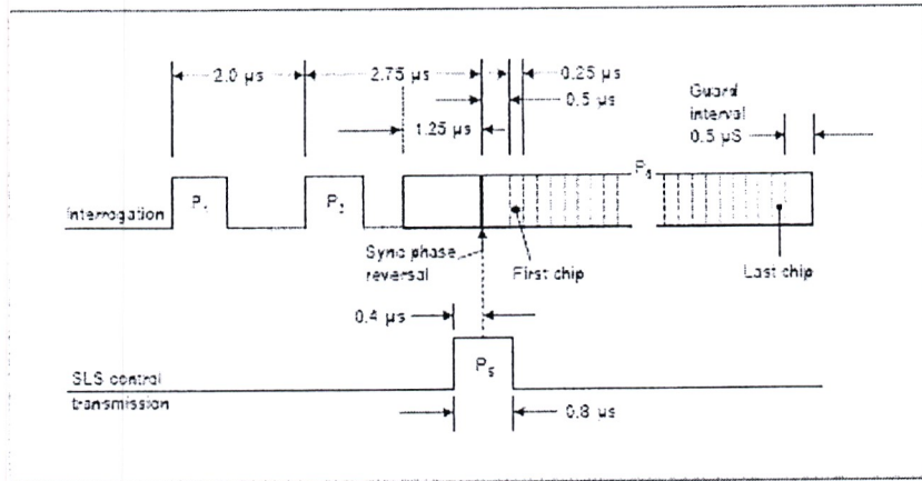
Figure 3-4. Mode S interrogation pulse sequence
