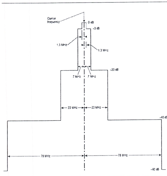
FIGURE 1-14: REQUIRED SPECTRUM LIMITS FOR TRANSPONDER TRANSMITTER--
