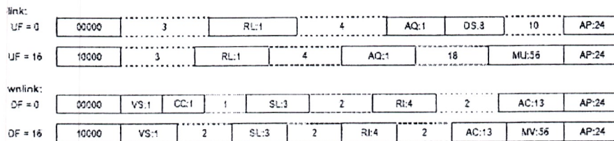
Figure 6-1: Surveillance and Communication formats used by ACAS
