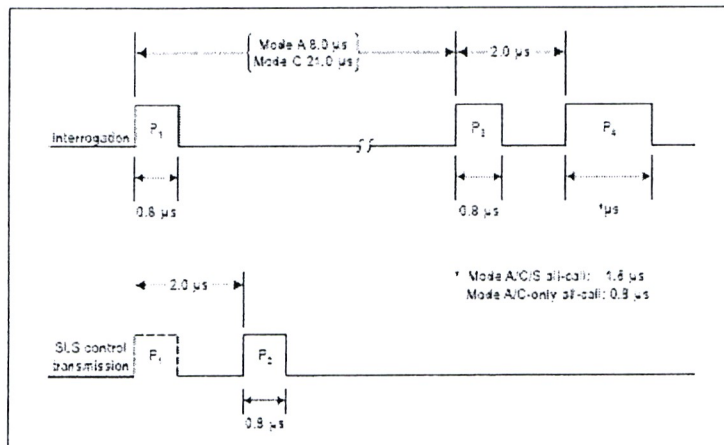
Figure 3-3. Intermode interrogation pulse sequence
