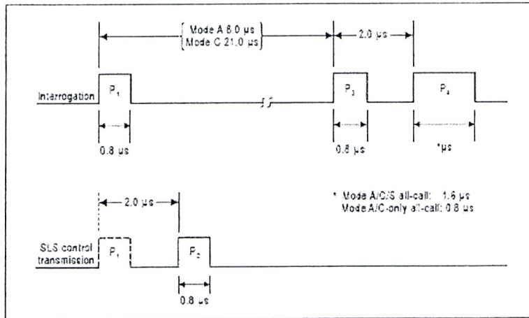
FIGURE 1-12: INTERMO DE INTERROGATION PULSE SEQUENCE
