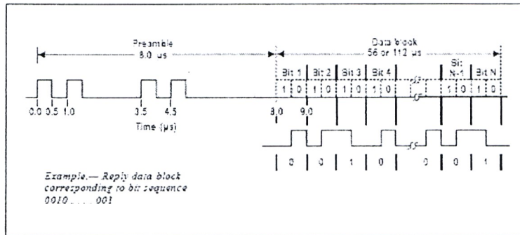
Figure 3-6. Mode S reply
