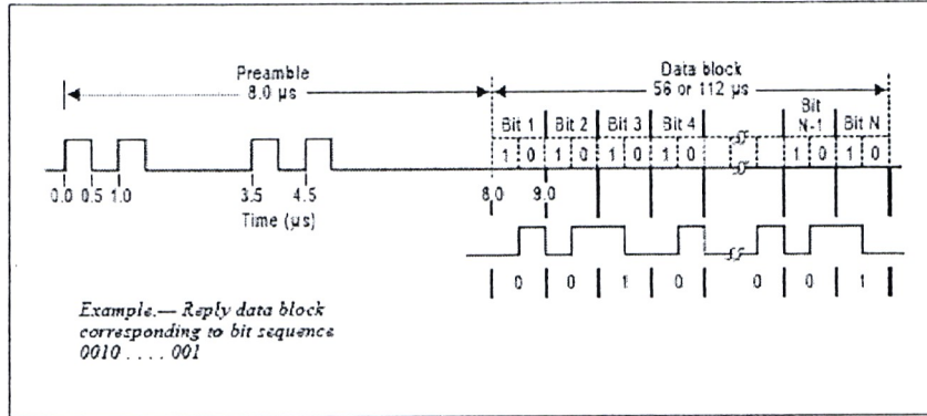
FIGURE 1.16: SUMMARY OF MODE S INTERROGATION OR UPLINK FORMATS
